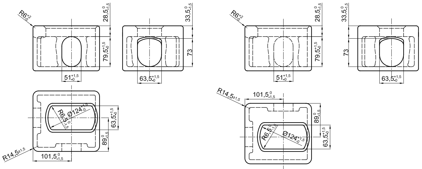
Bottom corner fitting
