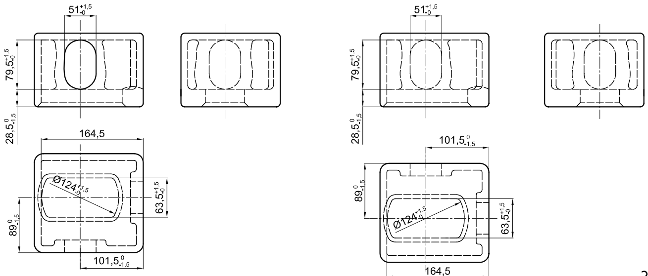
Bottom corner fitting
